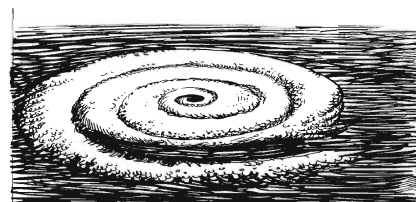
Fig-4.5: Cyclone
